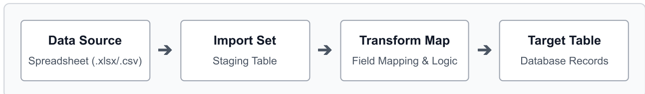
Figure 1: Architecture and data flow of the Import Data Using Transform Maps (Spreadsheet) application
